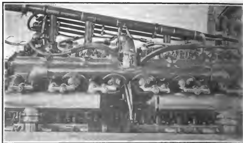
Left side of Rolls-Royce engine
